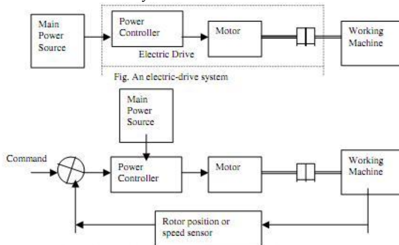
Fig. Modern Electric Drive system using power electronic converter
